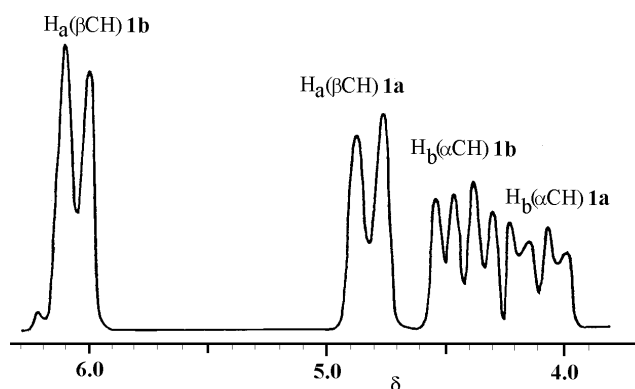
Fig. 1 ^1\text{H} NMR spectrum of conversion of 1a to 1b
