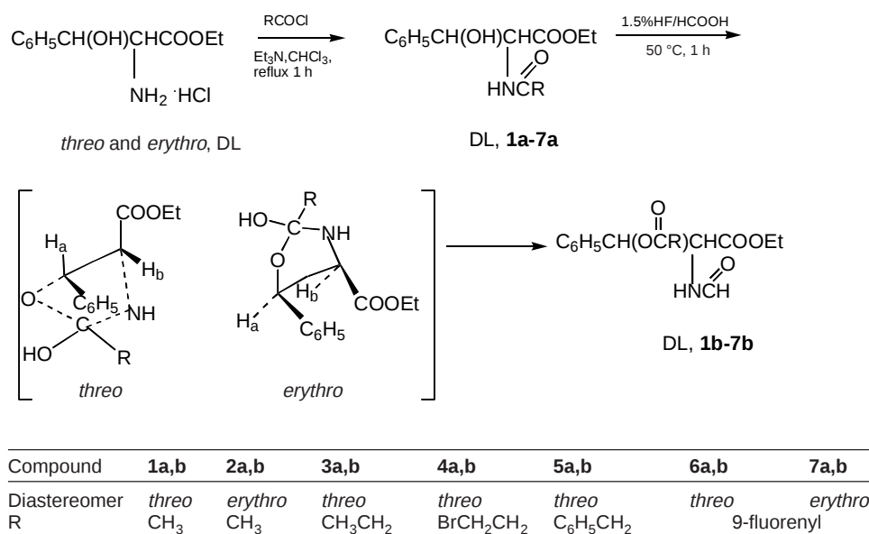
Scheme 1 Synthesis of N -formyl- O -acyl- threo -DL- \beta -phenylserines 1b–7b
